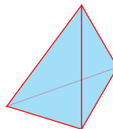
Tetraedro
